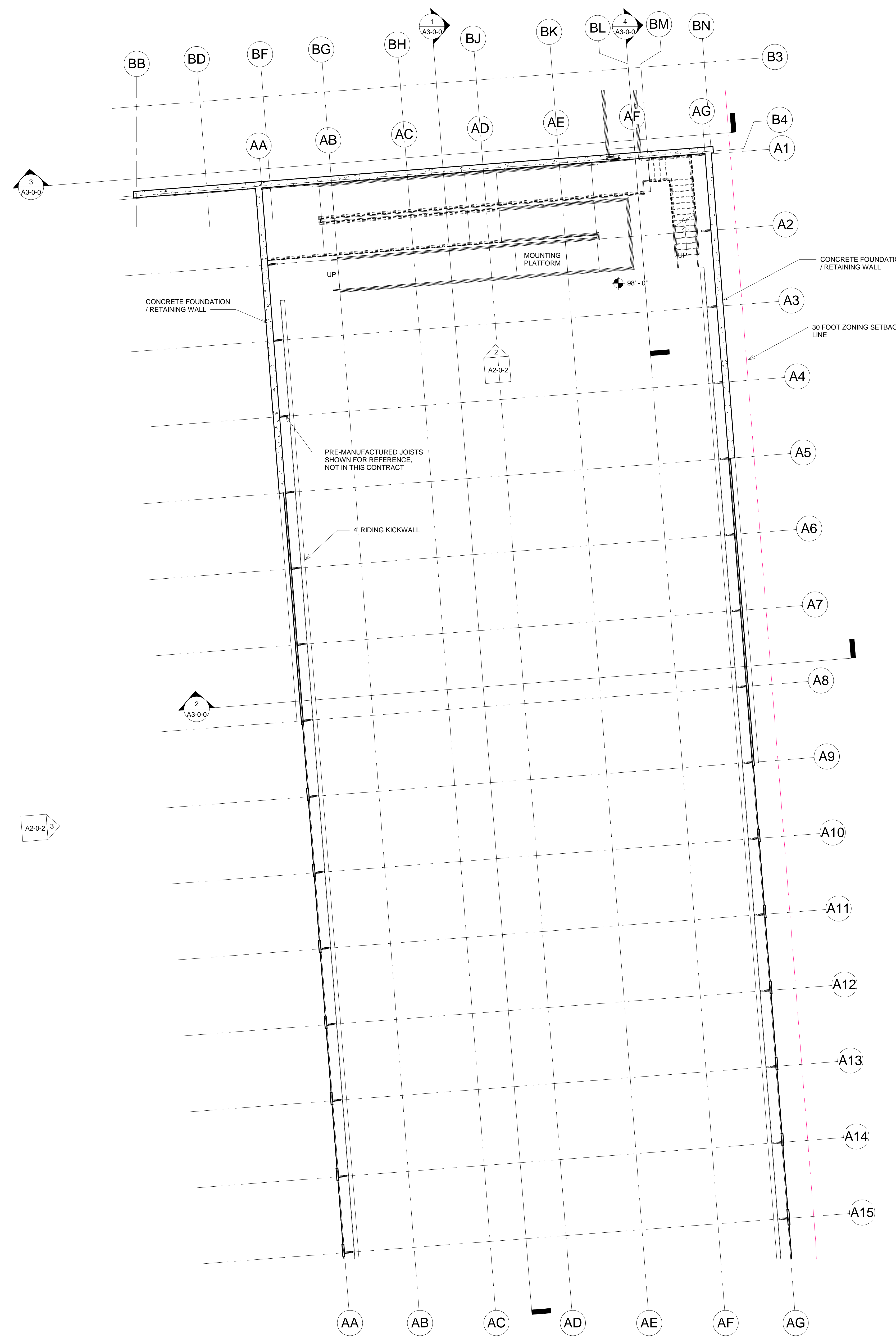
INDOOR RIDING ARENA LEVEL 1/8" = 1'-0"
