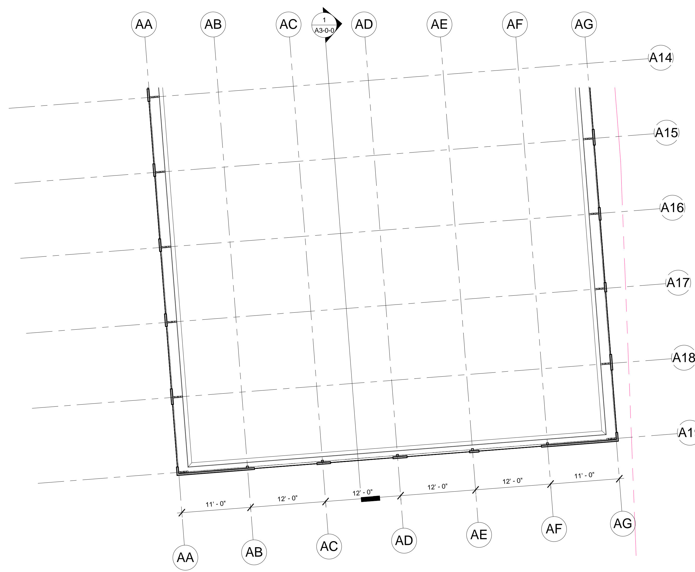
INDOOR RIDING ARENA LEVEL (SOUTH END) 1/8" = 1'-0"
